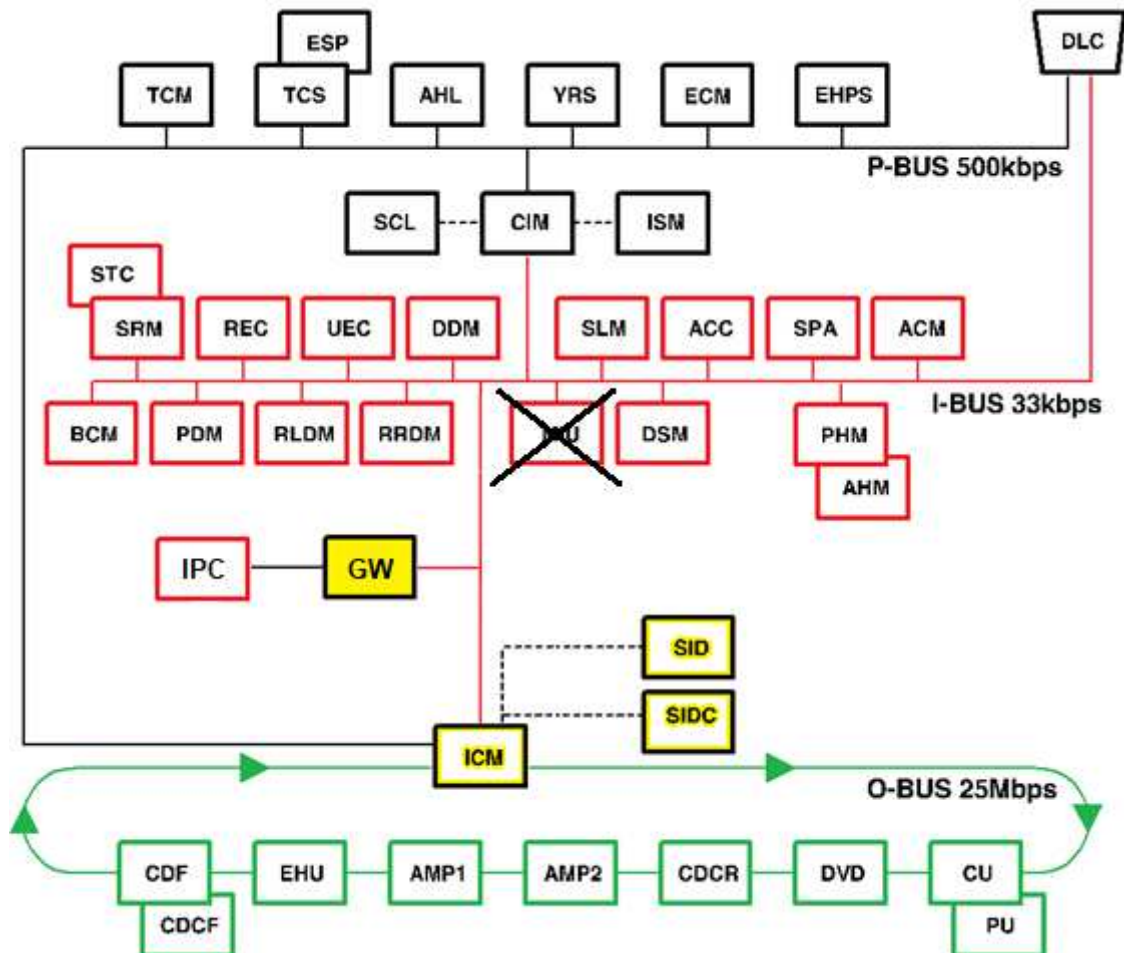
Saab 9-3 Electrical Architecture (2003-2006) with Saab NG9-5 IPC
