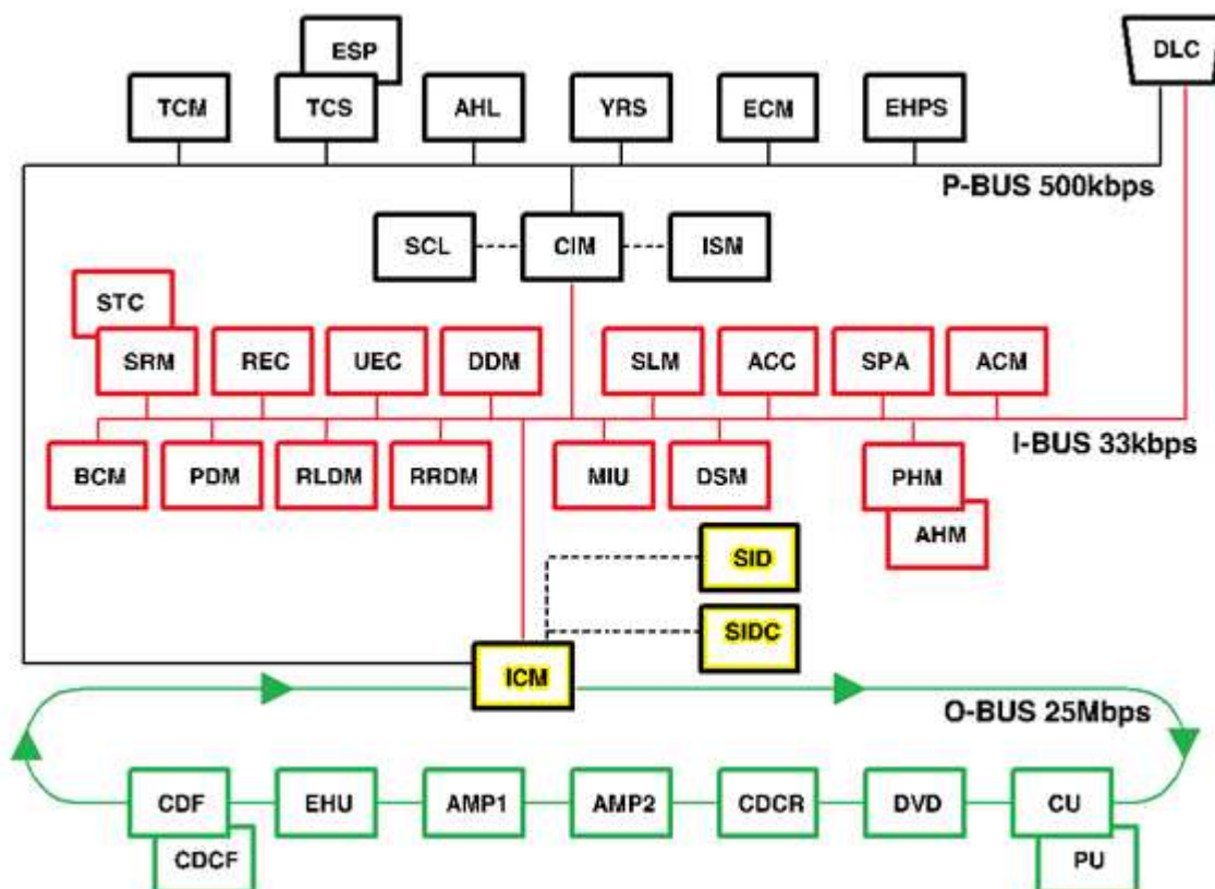
Saab 9-3 Electrical Architecture (2003-2006)
